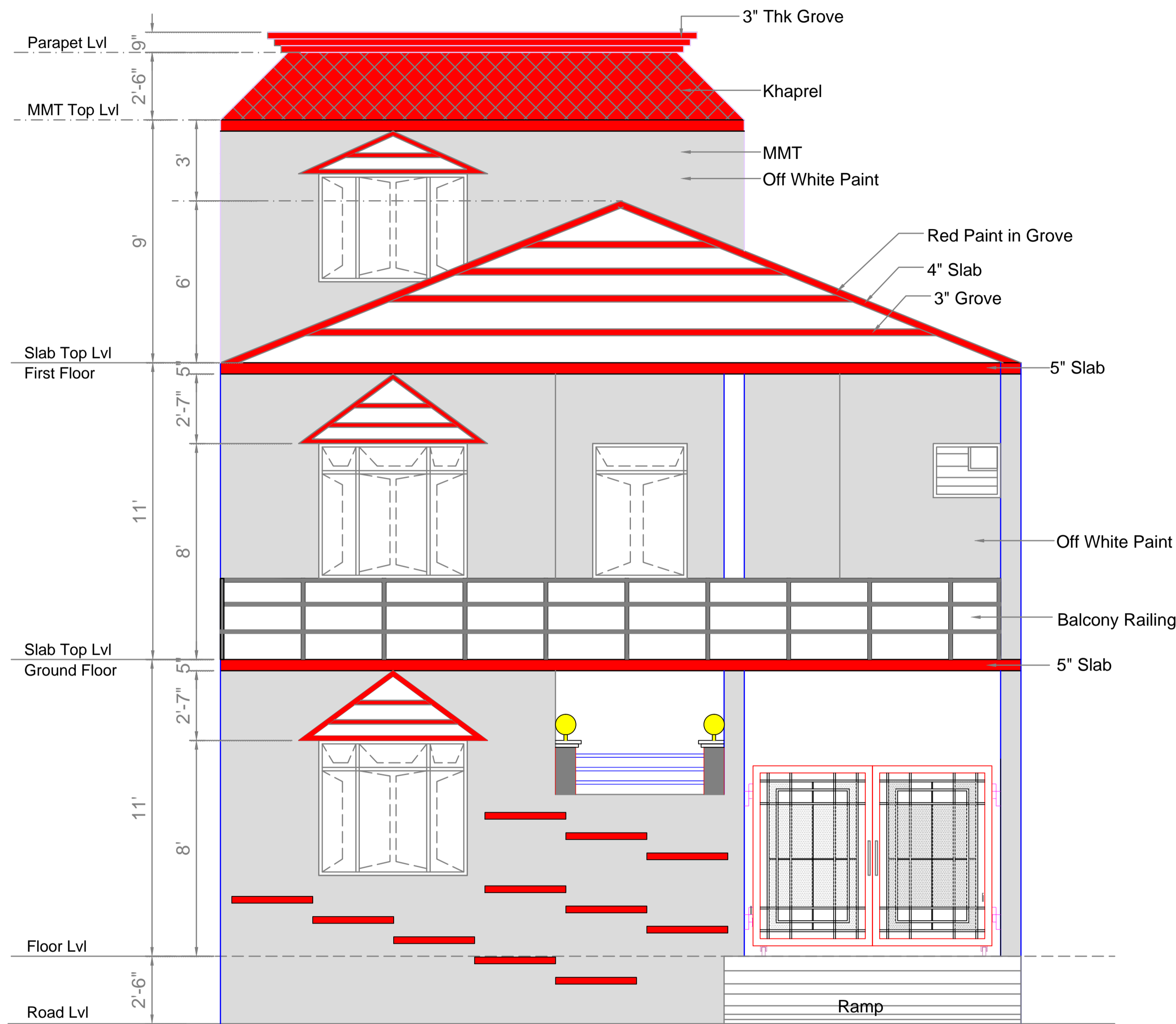
FRONT ELEVATION OPTION-I
