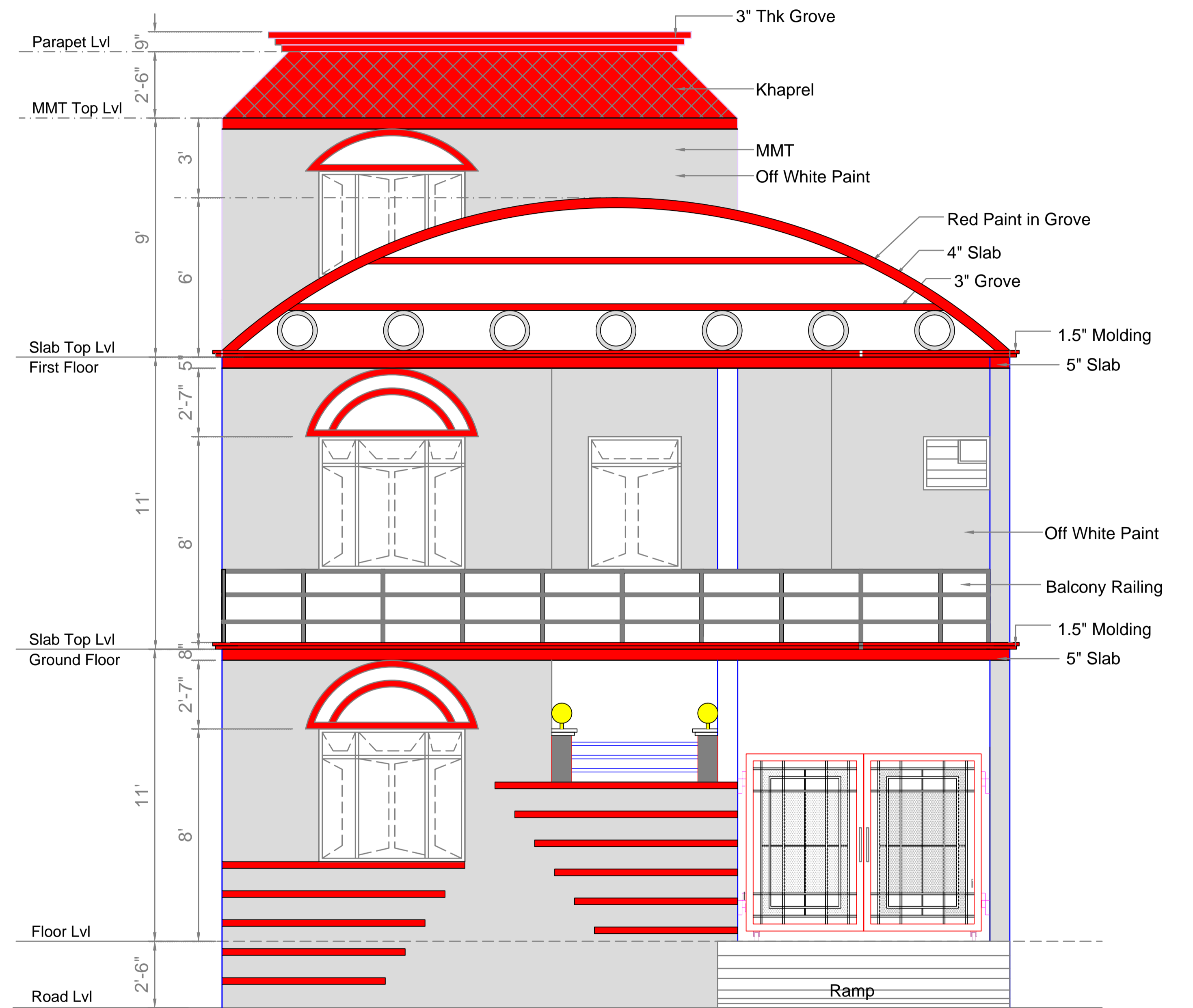
FRONT ELEVATION OPTION-II
